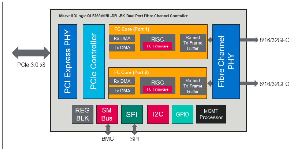
Figure 1. Marvell QLogic 2690 Series Adapters Block Diagram
